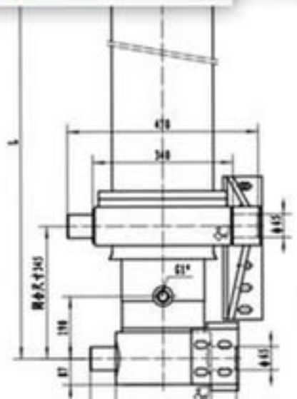
Abdominal lifting- HG160 Series Hydraulic cylinder
